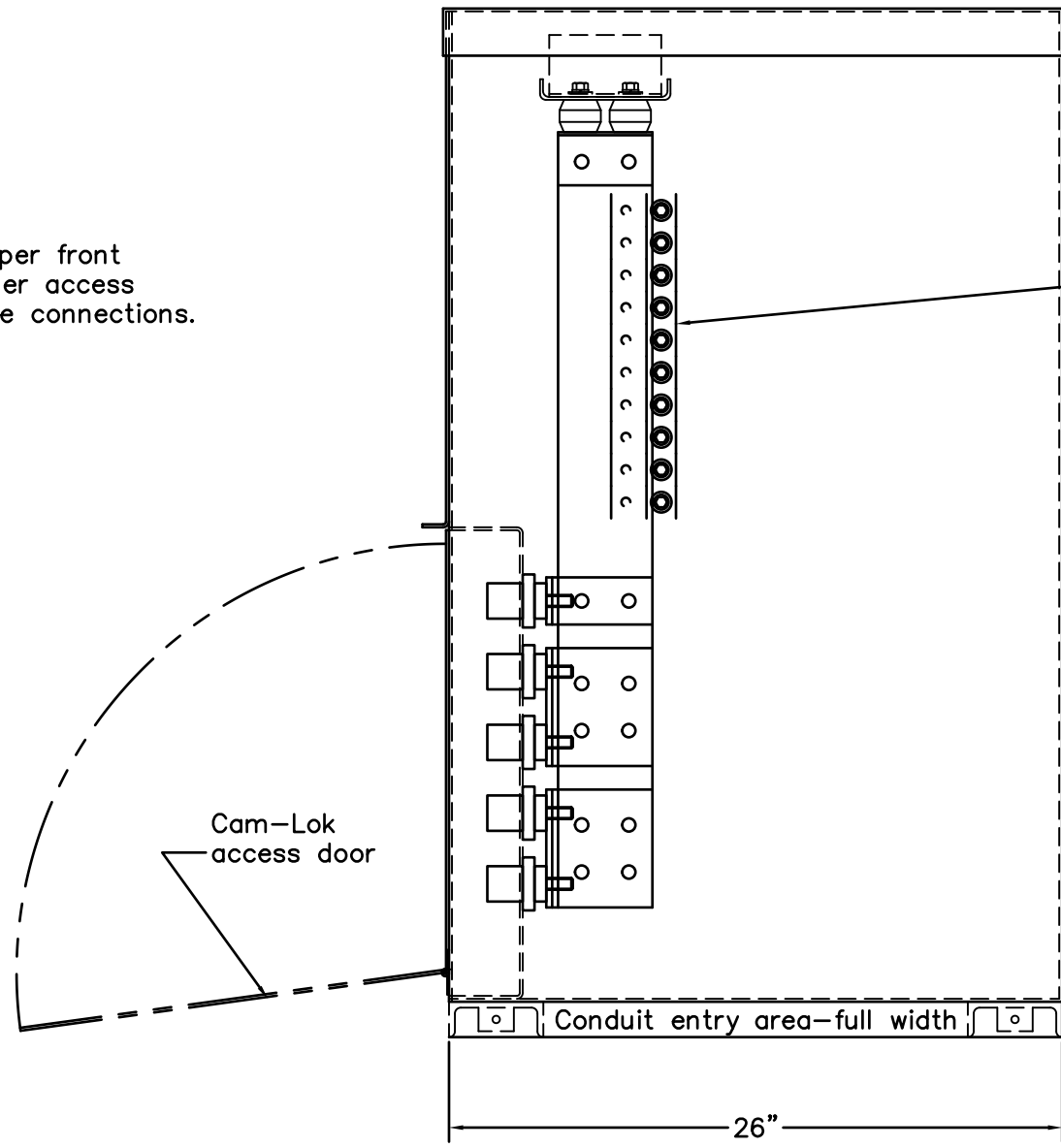
Right Side Cutaway Elevation View
