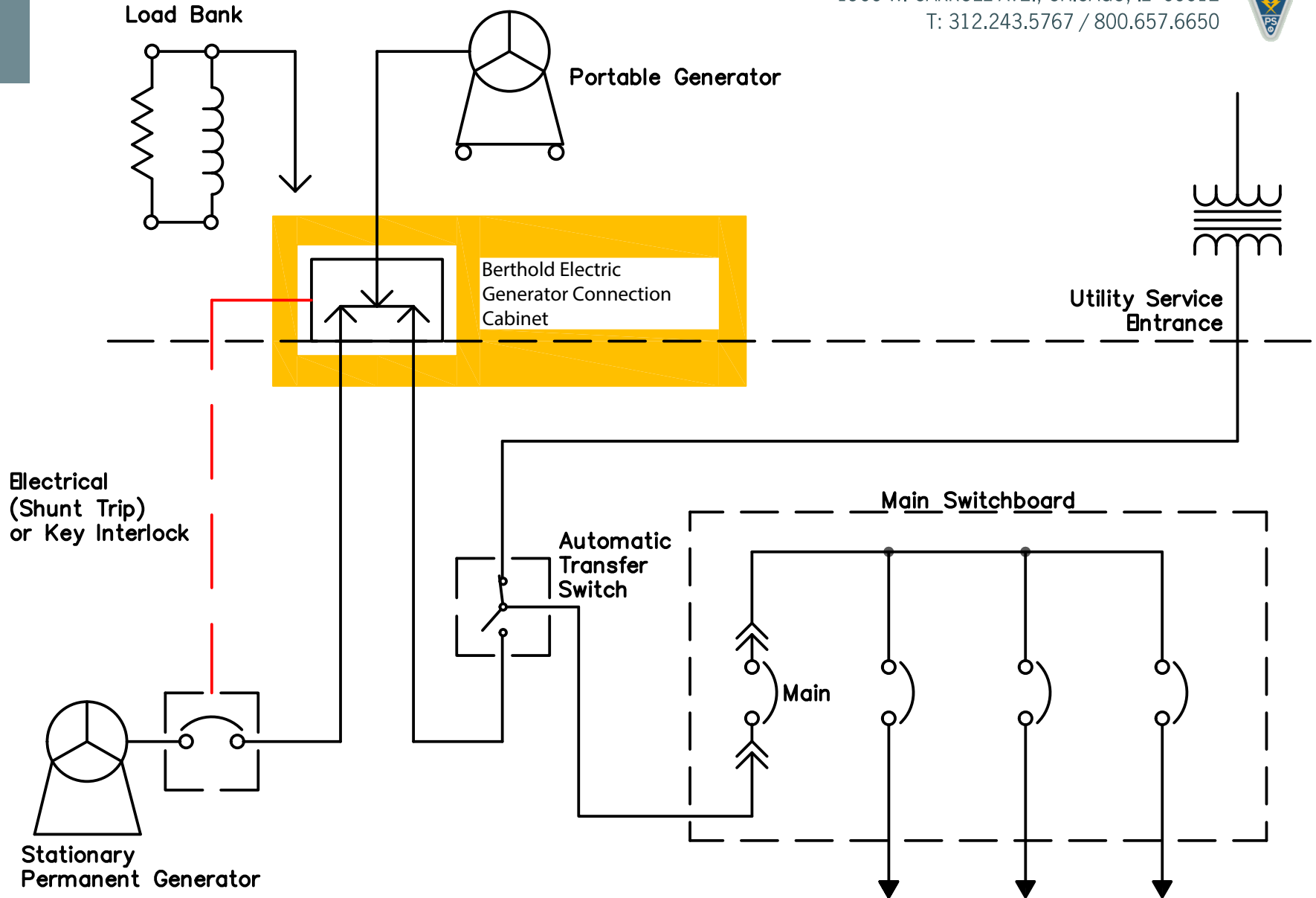
Permanent Generator With Transfer Switch Connect Portable Generator or Load Bank
