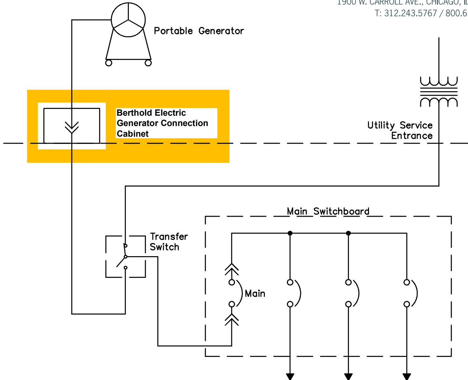
Portable Generator With Transfer Switch
