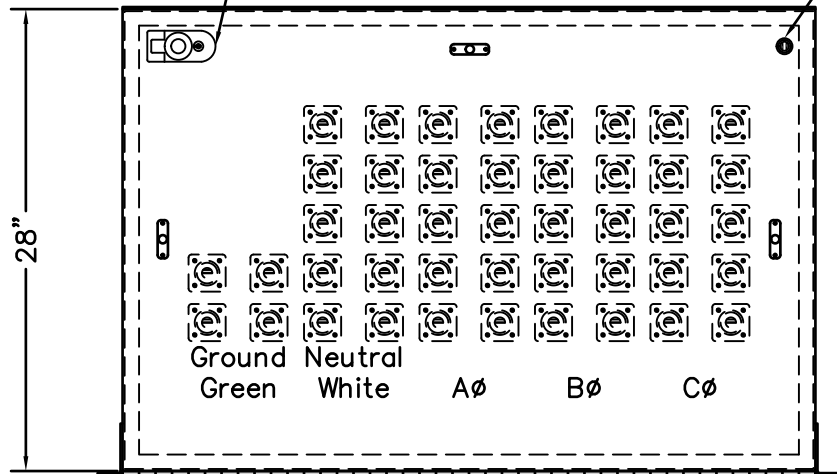
Bottom View (looking up)
