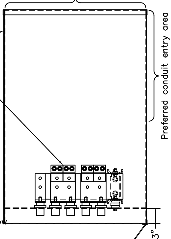
Right Side Elevation View
